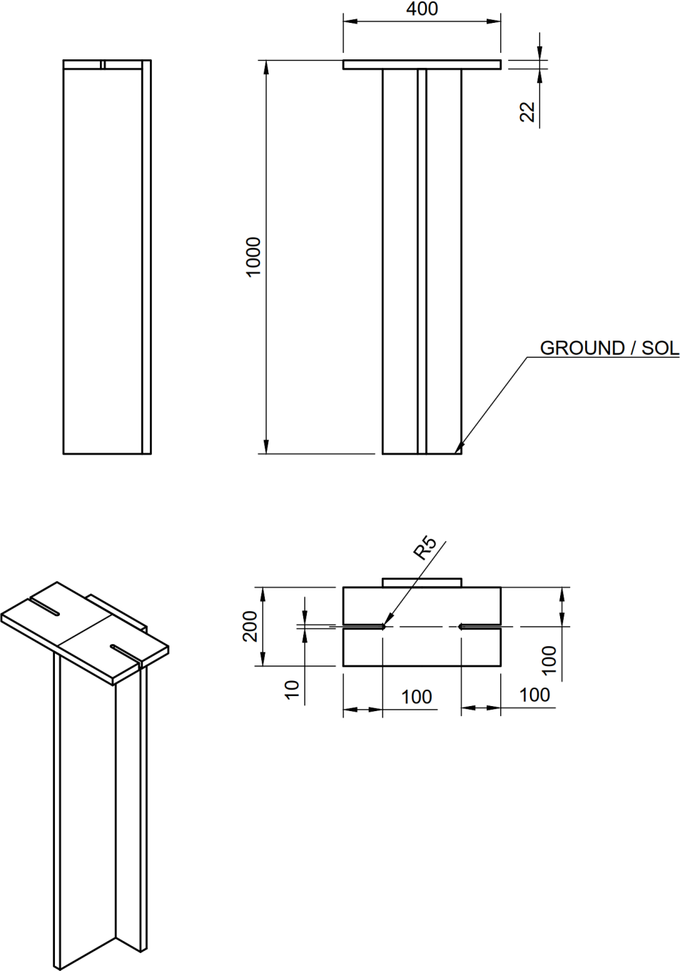
FIGURE 31 – Support de balise centrale
